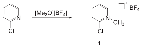
Scheme 1. Alkylation of chloropyridines according to Stone. [12]
