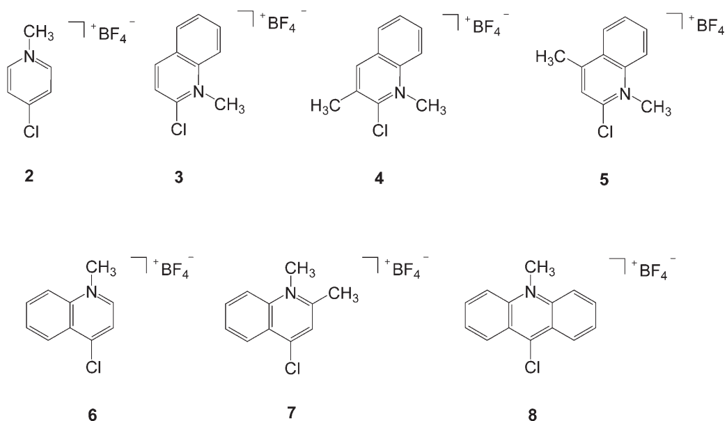
Figure 1. New ligand precursors 2–8 .
