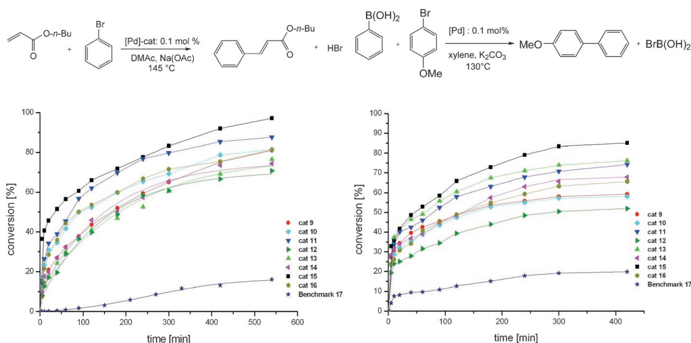
Figure 8. Time-conversion curves: Mizoroki–Heck reaction.
