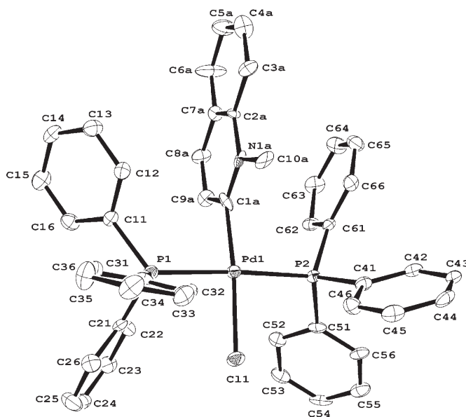
Figure 6. Molecular structure of cationic complex in 11-trans , showing the crystallographic numbering scheme (hydrogens and \text{BF}_4^- counteranion omitted for clarity).
