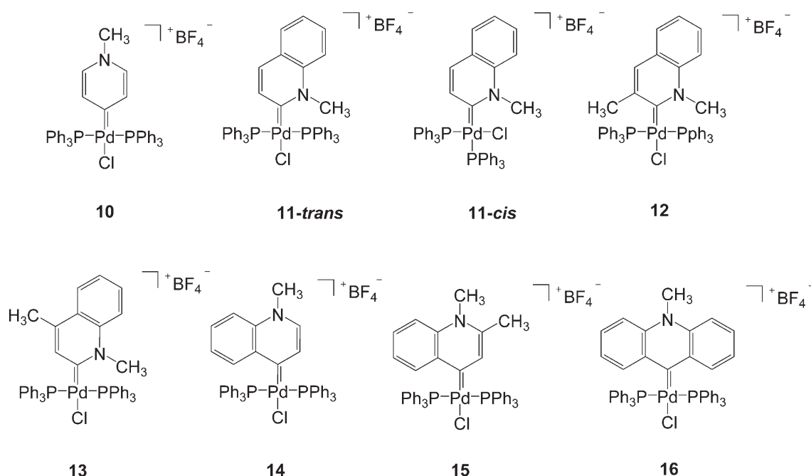
Figure 2. Carbene complexes 10–16.
