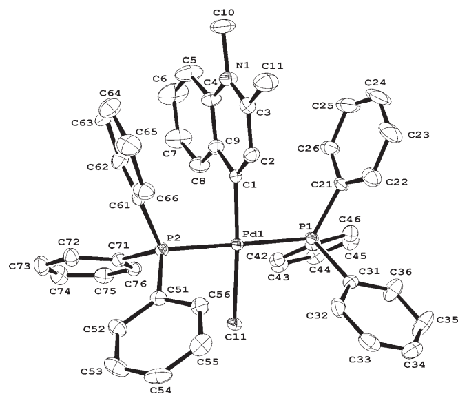
Figure 7. Molecular structure of the cationic complex in 15 , showing the crystallographic numbering scheme (hydrogens and \text{BF}_4^- counteranion omitted for clarity).
