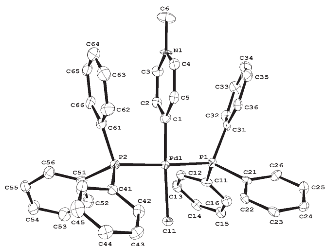
Figure 4. Molecular structure of the r NHC complex 10 , showing the crystallographic numbering scheme (hydrogens and \text{BF}_4^- counteranion omitted for clarity).
