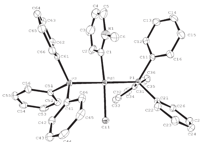
Figure 3. Molecular structure of the NHC complex in 9, showing the crystallographic numbering scheme (hydrogens and \text{BF}_4^- counteranion omitted for clarity).
