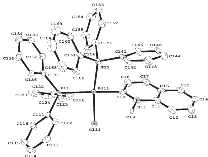
Figure 5. Molecular structure of the cationic complex in 11-cis , showing the crystallographic numbering scheme (hydrogens and \text{BF}_4^- counteranion omitted for clarity).
