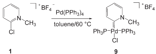
Scheme 2. Synthesis of complex 9 by oxidative addition.
